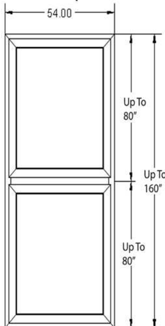
Stacked Twin Unit Equal Vent Integral Mullion
