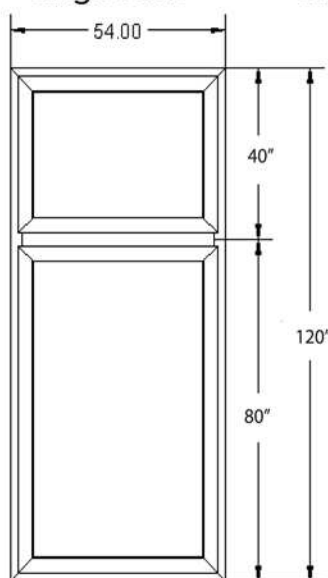
Stacked Twin Unit Un-Equal Vent Integral Mullion
